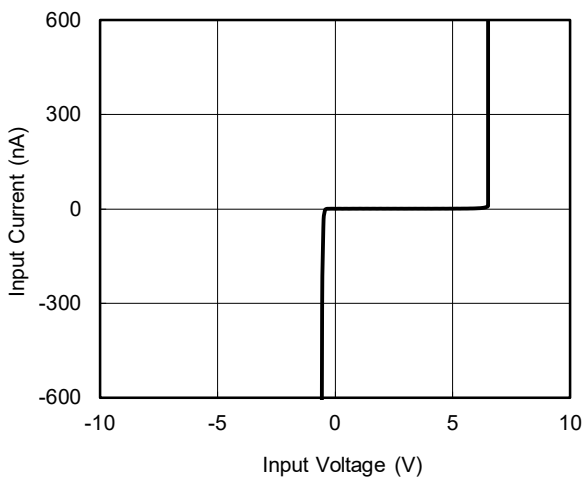
IV Curve
