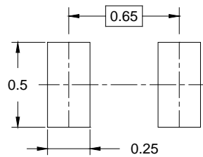
RECOMMENDED LAND PATTERN (Unit: mm)
