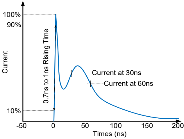
ESD pulse waveform per IEC 61000-4-2
