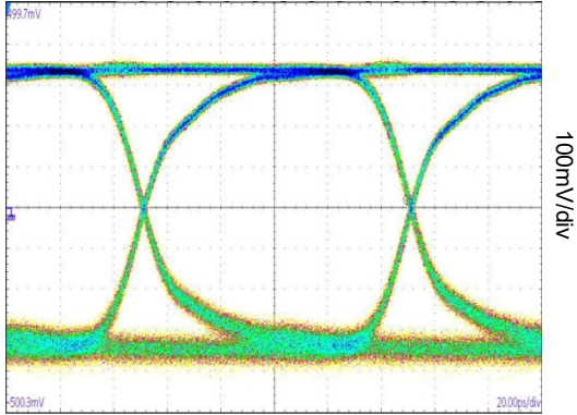
Time (20ps/div)
