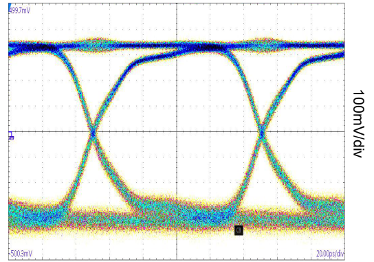
Time (20ps/div)
