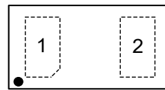
XTDFN-0.6×0.3-2L
