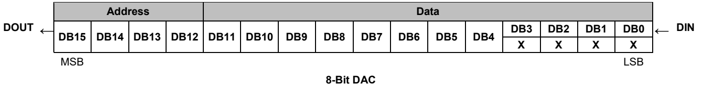
Figure 1. Serial Data
