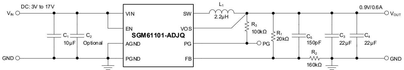
Figure 5. 0.9V Output Voltage Application of SGM61101-ADJQ
