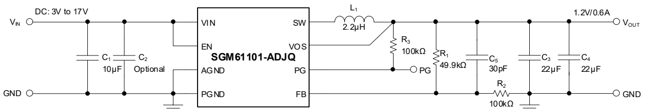
Figure 6. 1.2V Output Voltage Application of SGM61101-ADJQ
