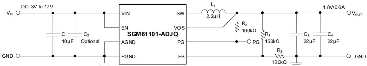
Figure 7. 1.8V Output Voltage Application of SGM61101-ADJQ
