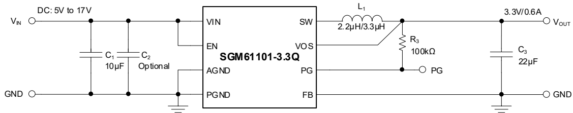
Figure 9. Application of SGM61101-3.3Q
