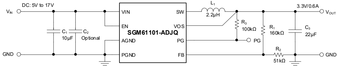
Figure 4. 3.3V Output Voltage Application of SGM61101-ADJQ
