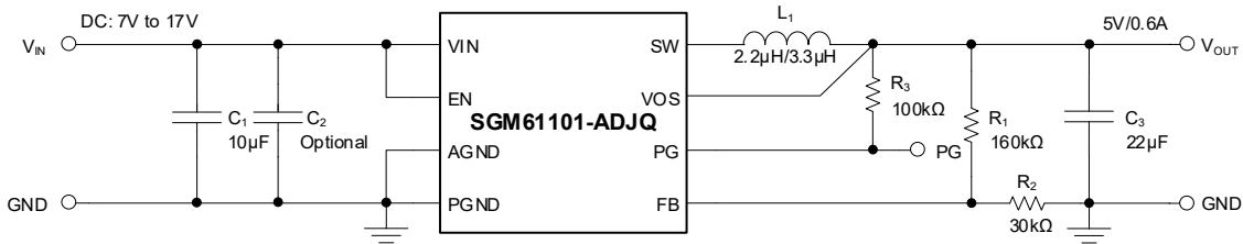
Figure 8. 5V Output Voltage Application of SGM61101-ADJQ
